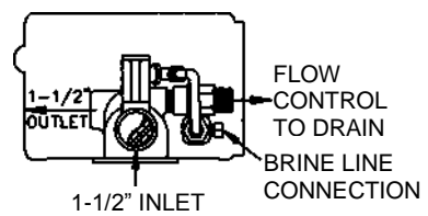
REAR VIEW OF 2850 VALVE
