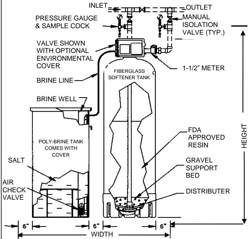
FRONT VIEW OF SINGLE WATER SOFTENER
