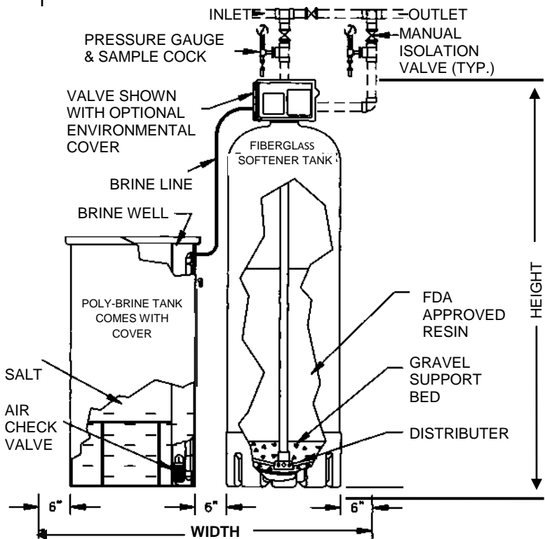
FRONT VIEW OF SINGLE WATER SOFTENER
