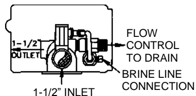
REAR VIEW OF 2850 VALVE
